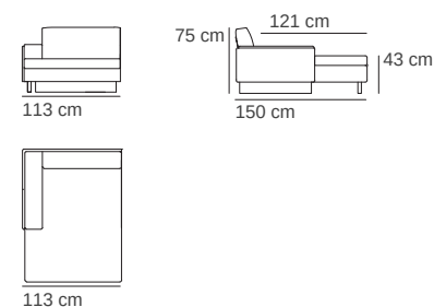
113W × 150D × 75H cm mt 8.79 | 1.2 m³ | 58 kg Chaise Lounge Cod. 118
