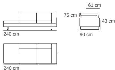
240W × 90D × 75H cm mt 16.61 | 1.5 m³ | 79 kg Corner Cod. 293
