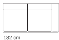
182W × 90D × 75H cm mt 12.96 | 1.17 m³ | 62 kg Module Cod. 147
