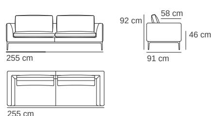
255W × 91D × 92H cm mt 15.3 | 1.99 m³ | 84 kg Sofa Cod. 296
