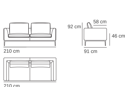
210W × 91D × 92H cm mt 15.15 | 1.65 m³ | 73 kg Sofa Cod. 045
