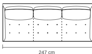
247W cm 3-seater Sofa Cod. ANTD247
