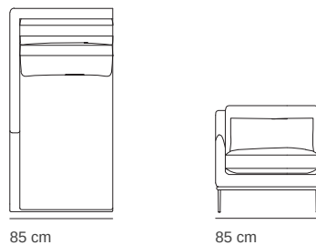
85W × 168D × 88H cm mt 12.69 | 1.19 m³ | 45 kg Chaise Lounge Cod. 019
