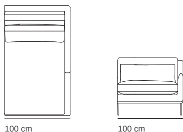
100W × 168D × 88H cm mt 12.71 | 1.38 m³ | 48 kg Chaise Lounge Cod. 119
