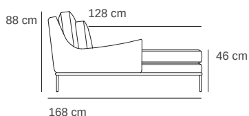
85W × 168D × 88H cm mt 12.69 | 1.19 m³ | 45 kg Chaise Lounge Cod. 018
