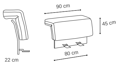
90W × 22D × 45H cm mt 2.2 + 1.5 | 0.22 m³ | 13 kg Low Slim Back Set Cod. QHBB3
