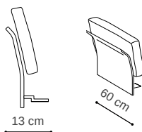
62W × 13D × 32H cm mt 1 + 0.8 | 0.17 m³ | 8 kg Low Slim Back & Armrest Cushion Cod. QHBC1
