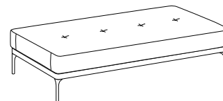
182W × 82D × 43H cm mt 4.4 | 0.47 m³ | 63 kg Base Cod. U2RI0
