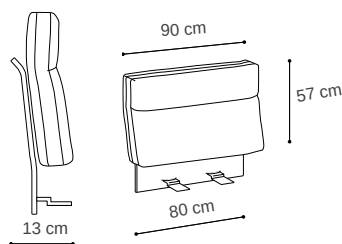
90W × 13D × 57H cm mt 2.1 + 1.9 | 0.22 m³ | 13 kg High Slim Back Set Cod. QHAA3
