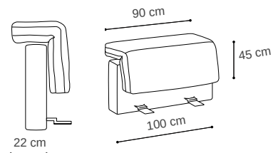
100W × 22D × 45H cm mt 2.2 + 1.6 | 0.25 m³ | 17 kg Back Cushion Set Cod. QHIB3
