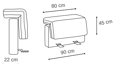
90W × 22D × 45H cm mt 2.2 + 1.6 | 0.22 m³ | 15 kg Back Cushion Set Cod. QHIB2
