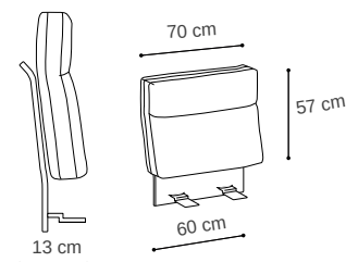
70W × 13D × 57H cm mt 2.1 + 1 | 0.17 m³ | 3 kg High Slim Back Set Cod. QHAA1
